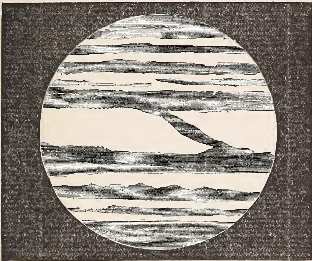
FIG. 3.—The Planet Jupiter (Browning).
